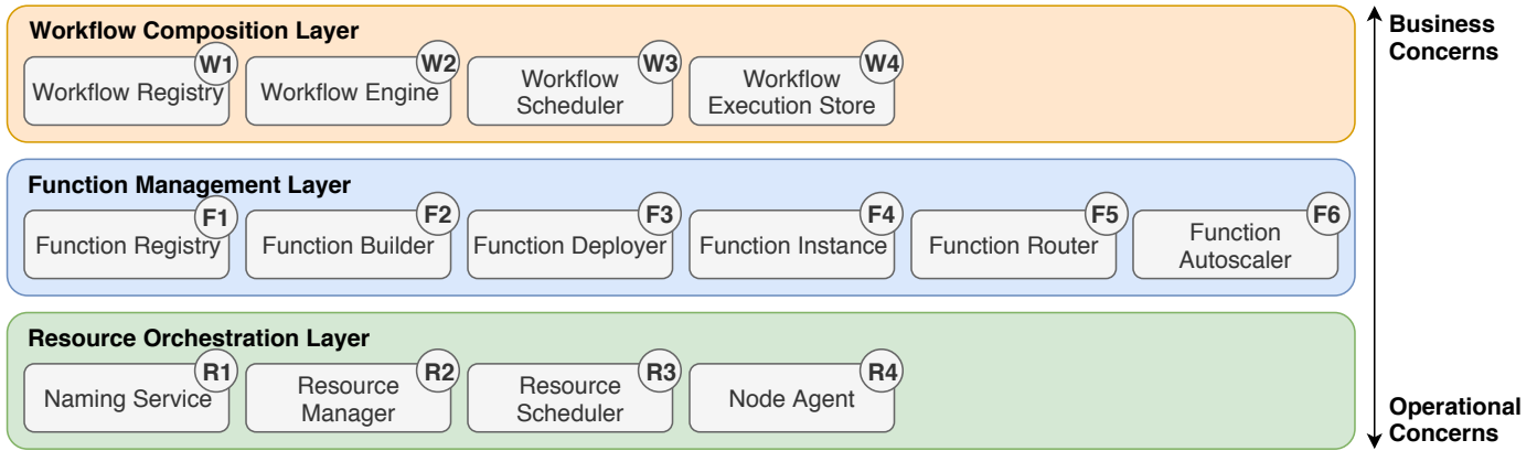
Fig. 1: The SPEC-RG reference architecture for FaaS platforms.
