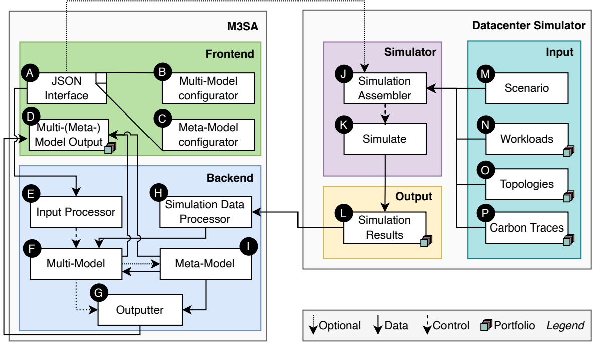
Figure 25: High-level architecture of M3SA integrated within a datacenter simulator.
