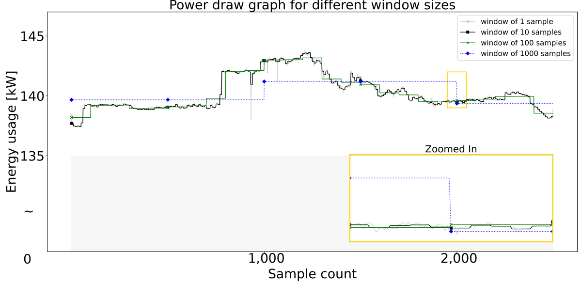
Figure 18: 2,500 simulation data entities, processed with 1, 10, 100, and 1,000 window sizes, leveraged in the same graph.
