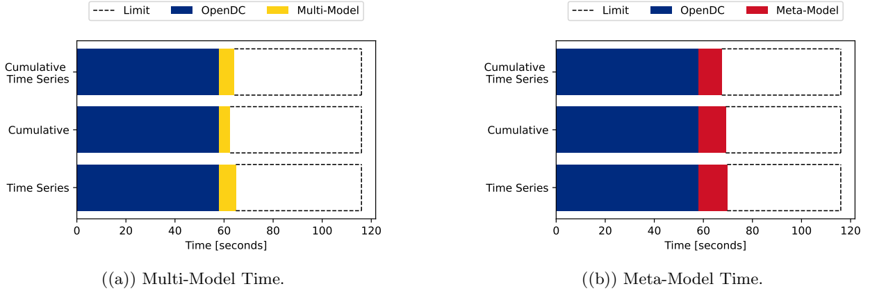
Figure 33: Individual performance evaluation, for Multi-Model and Meta-Model, applied to OpenDC, against the performance threshold.
