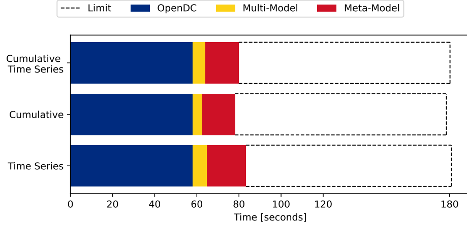
Figure 34: M3SA, applied to OpenDC, against the performance threshold.
