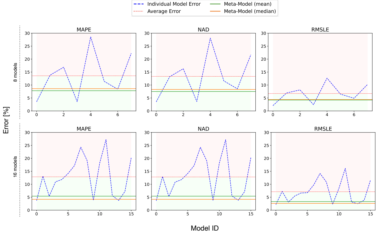
Figure 35: Accuracy validation for the Meta-Model using 8 and 16 individual models, evaluated using MAPE, NAD, and RMSLE metrics.
