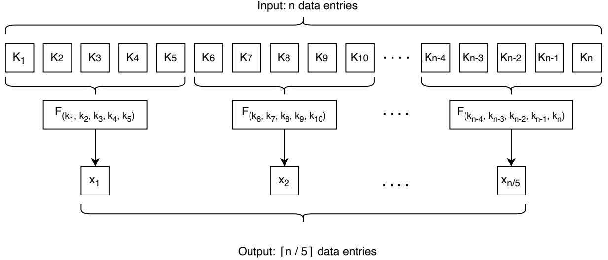
Figure 16: Window of size 5 applied on n data entries, using function F as aggregation function.
