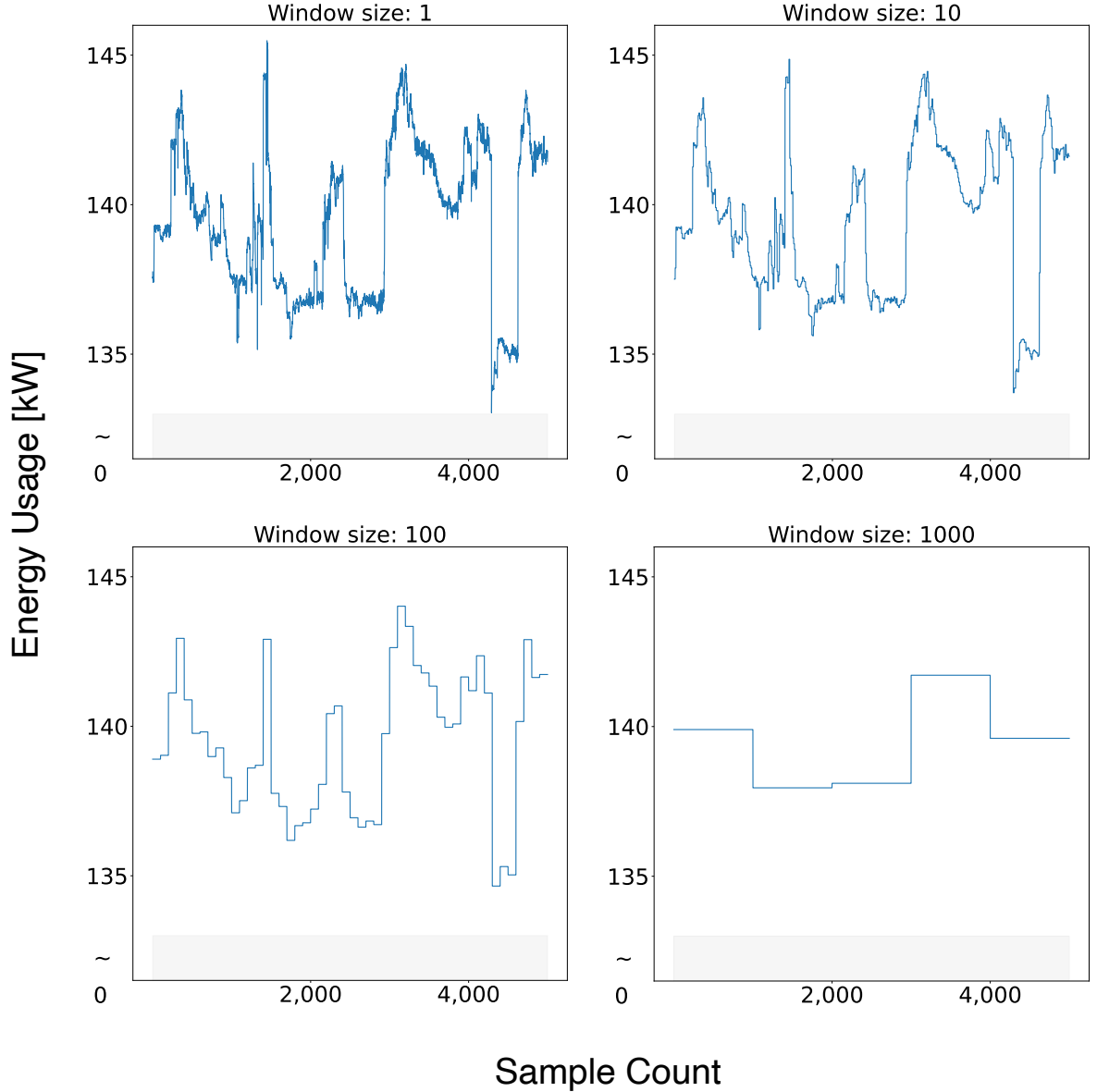
Figure 17: 5,000 simulation data entities plotted with window sizes of 1, 10, 100, and 1,000.
