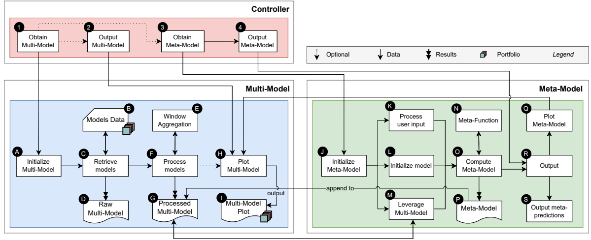
Figure 29: Meta-Model embedded within the Multi-Model.
