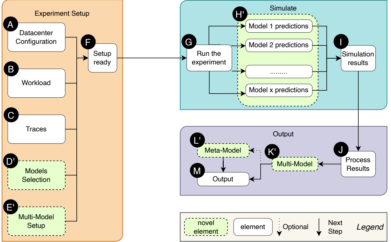
Figure 14: Simulation using multiple models. The proposed state-of-the-art.
