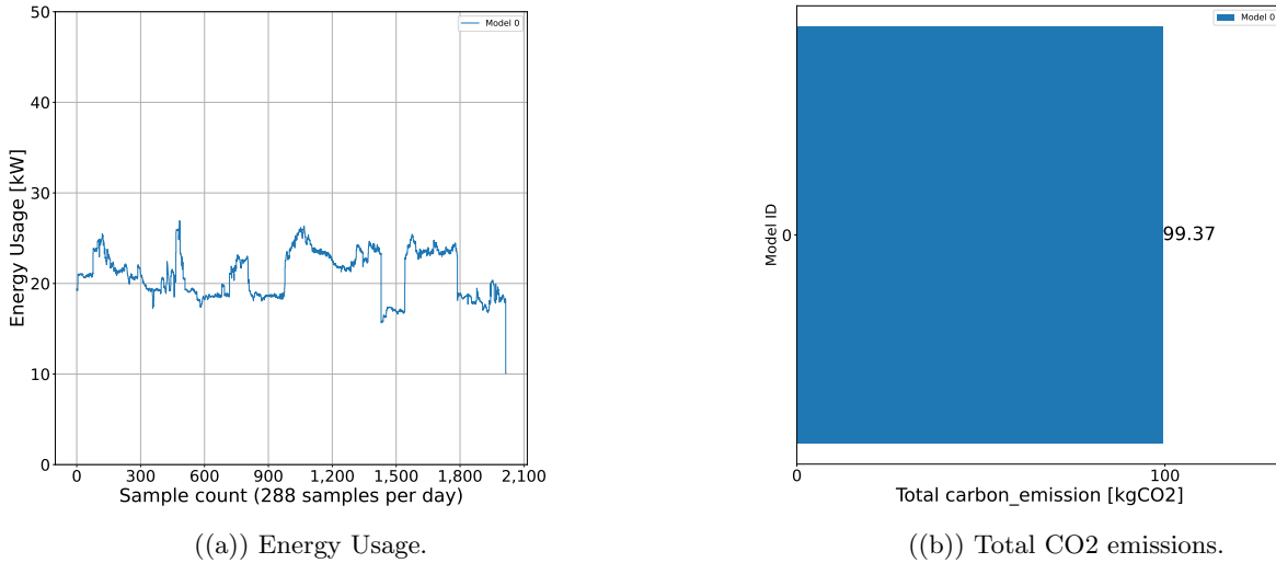
Figure 36: M3SA predictions for the scaled infrastructure, using a single model.
