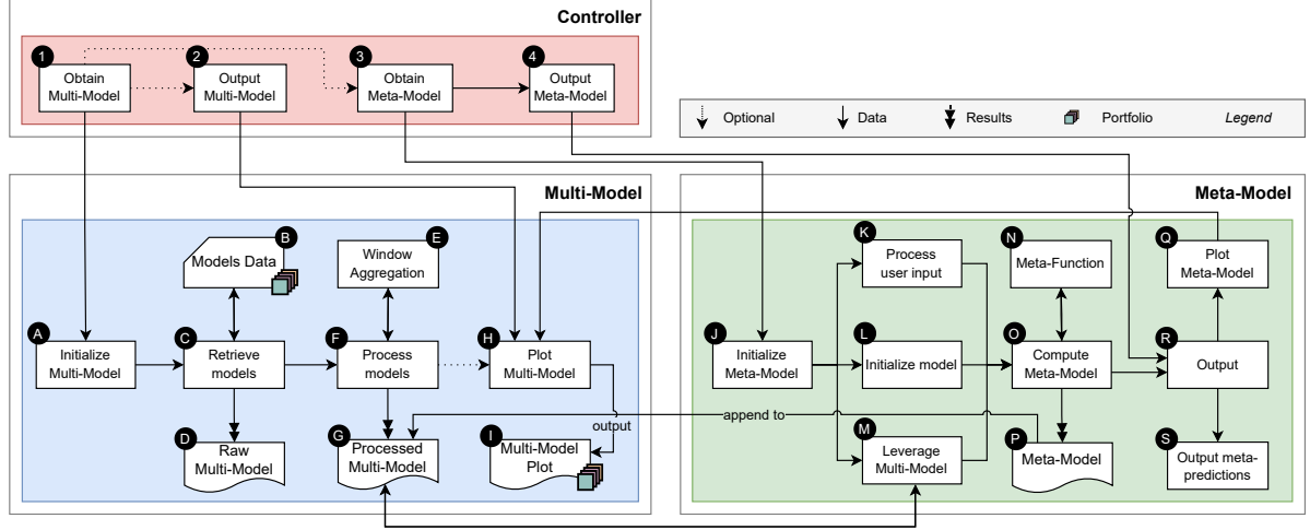
Figure 24: Meta-Model embedded within the Multi-Model.
