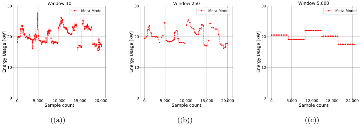
Figure 31: Three Meta-Models computed with window sizes of 10, 250, and 5000.
