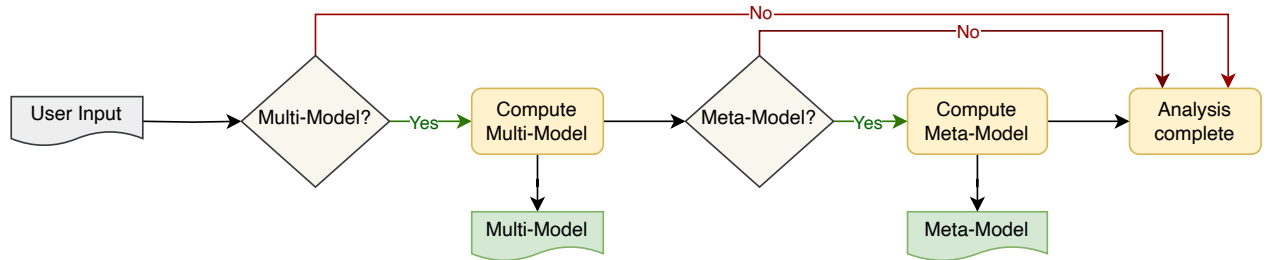
Figure 30: Decision flowchart for computing Multi-Model, Meta-Model, both, or none, based on user input.
