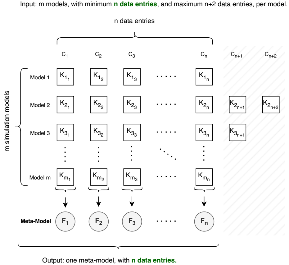
Figure 23: Meta-Model simulation concept.
