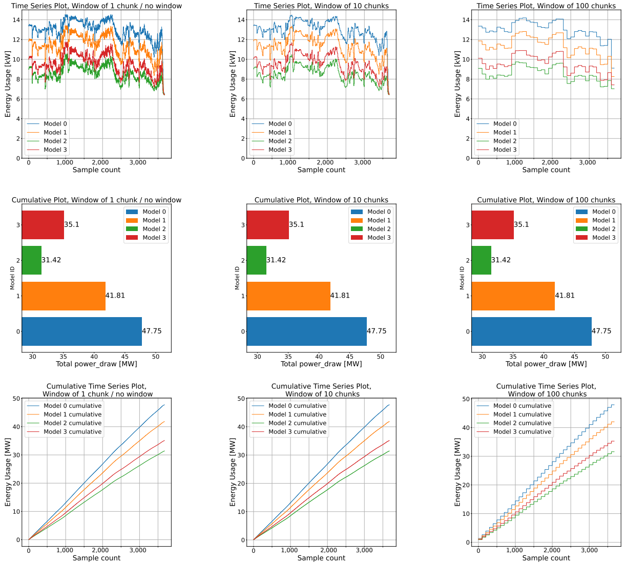
Figure 19: Multi-Model-supported plots, with 1, 10, and 100 window sizes.
