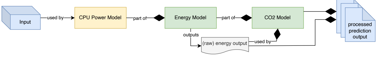
Figure 6: Prediction Architecture in OpenDC framework.
