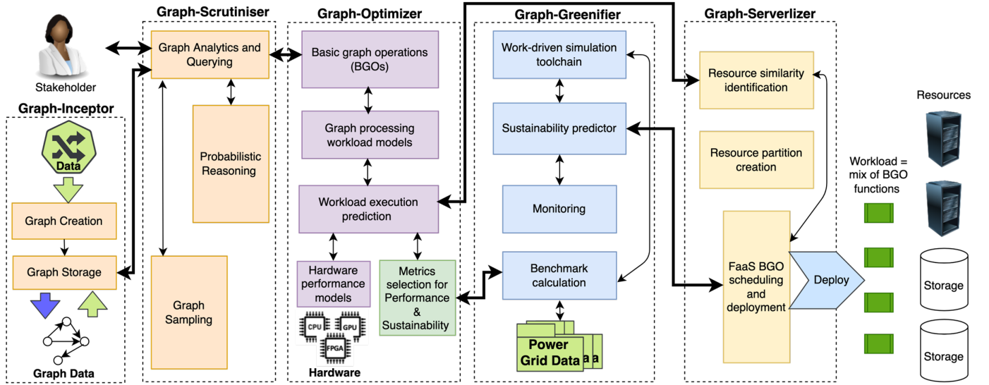
Fig. 2. Graph-Massivizer technical architecture.
