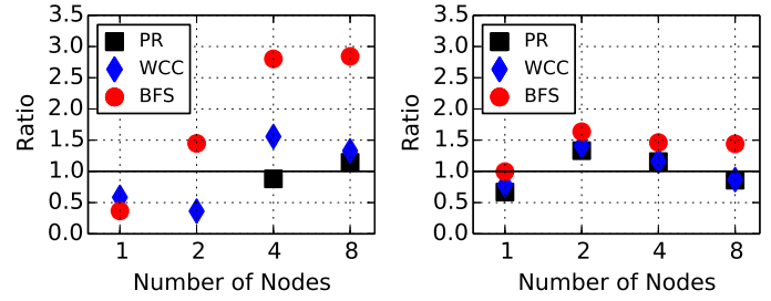
Fig. 11. Horizontal scalability analysis on KNL vs. Xeon running algorithms WCC, BFS, PR. Points depict the ratio of KNL: Xeon runtime. Lower is better for KNL. Dataset: G25. There are missing symbols: PR does not complete within 2hrs, on 1 and 2 nodes, for KNL and Xeon.
