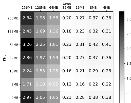
Fig. 6. GraphX block-size analysis, KNL vs. Xeon. Values in matrix represent the ratio of runtimes, KNL:Xeon. Algorithm: WCC. Dataset: G24. (Higher values are worse. For values above 1, KNL is slower than Xeon.)
