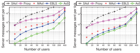
Fig. 4. Network upload: (left) the WI workload; (right) the WD workload. (Logarithmic scale on vertical axes).
