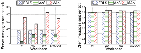
Fig. 6. Network upload, 60 users: (left) server; (right) client. (For the servers' upload of AoS and AoI, each bar is divided into 3 parts, from top to bottom (dark, gray, and light): number of commands sent, number of shared-zones' states sent, number of state-updates sent. Servers of EBLs only send commands, thus the bars for EBLs are not partitioned.)
