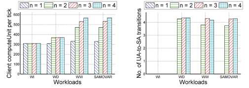
Fig. 9. Dynamic area management mechanism with increasing n : (left) client compute unit and (right) number of UA-to-SA transitions.
