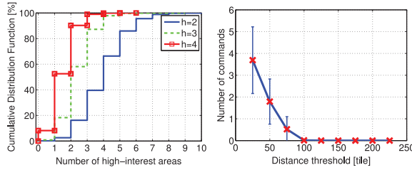
Fig. 2. The presence of multiple, changing AoI in MAVEs: number of high-interest areas per user (left) and dynamics of interest (right).
