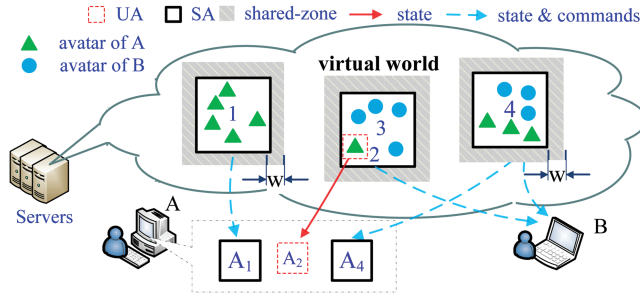
Fig. 3. A game map and overlapping simulation areas (SA) and update areas (UA). w is the width of the shared-zone.
